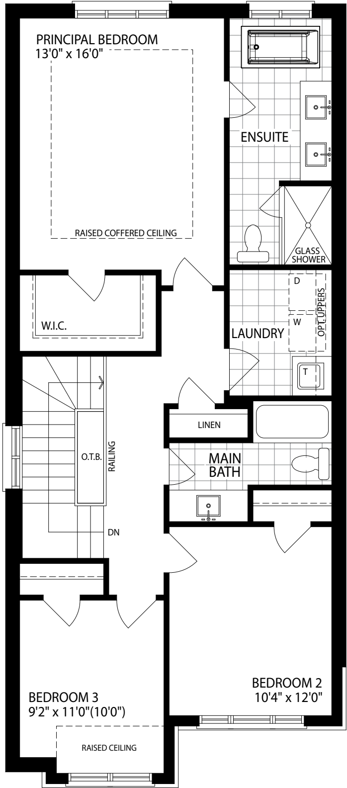
UPPER FLOOR ELEV. A
