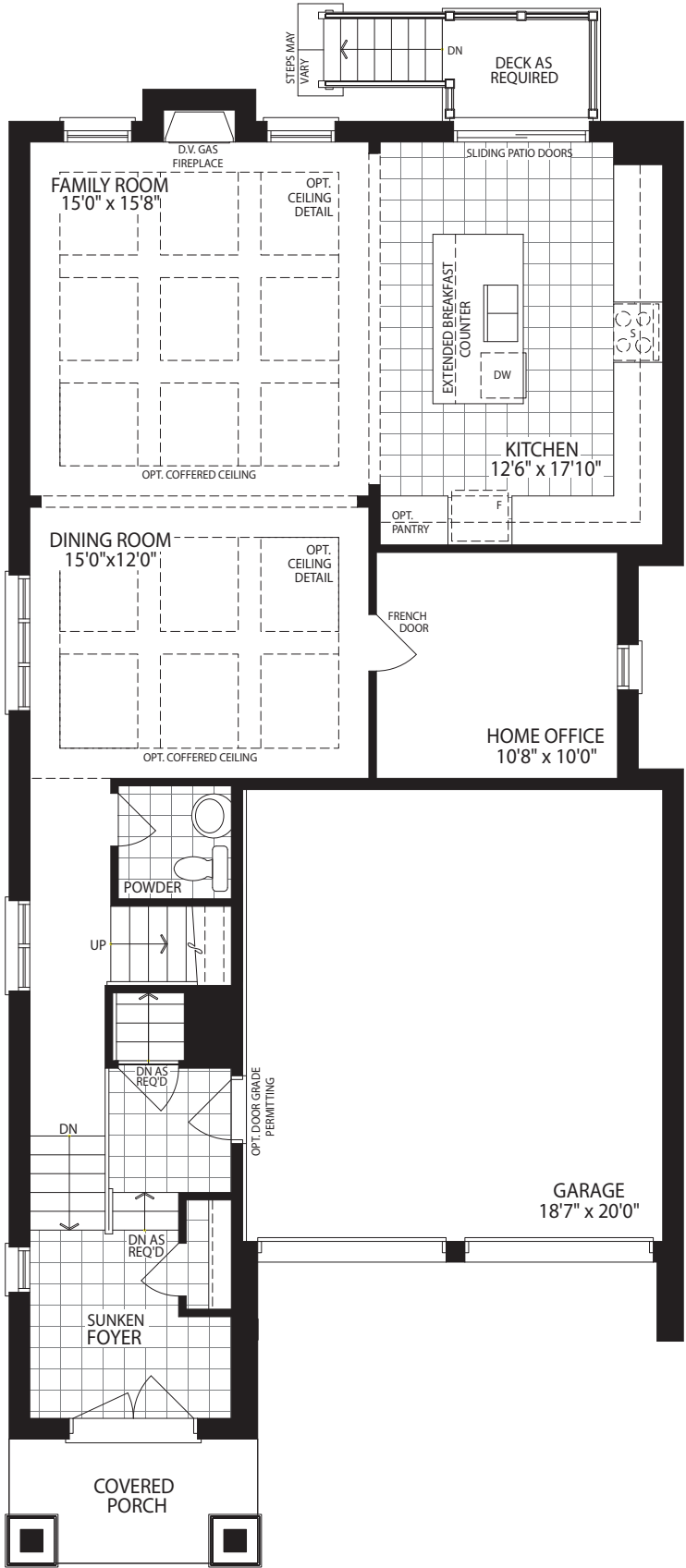
MAIN FLOOR ELEV. A
