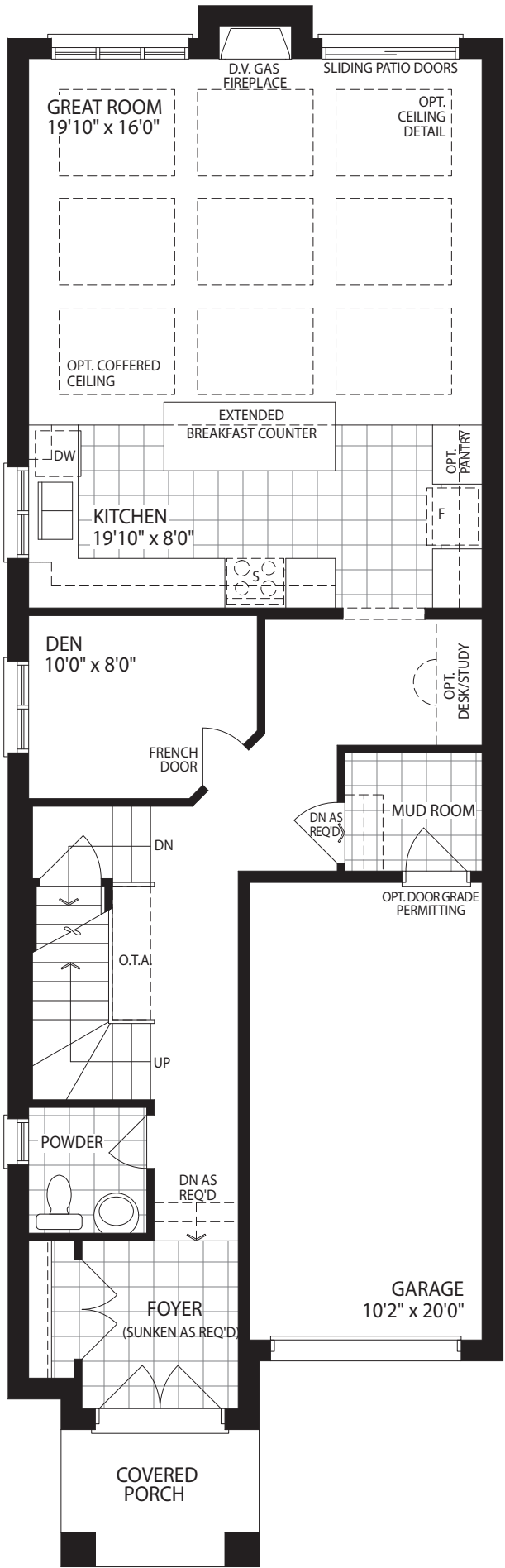
MAIN FLOOR ELEV. A
